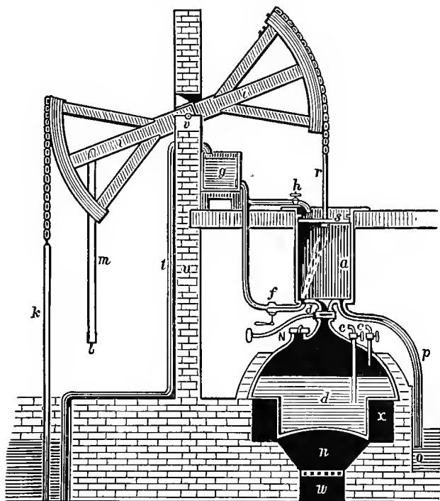
Newcomen's Steam Engine, 1704
